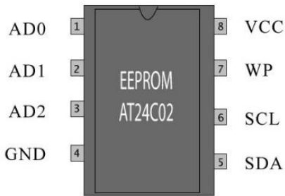
Figura 4: Diagrama de memoria eeprom AT24C02
